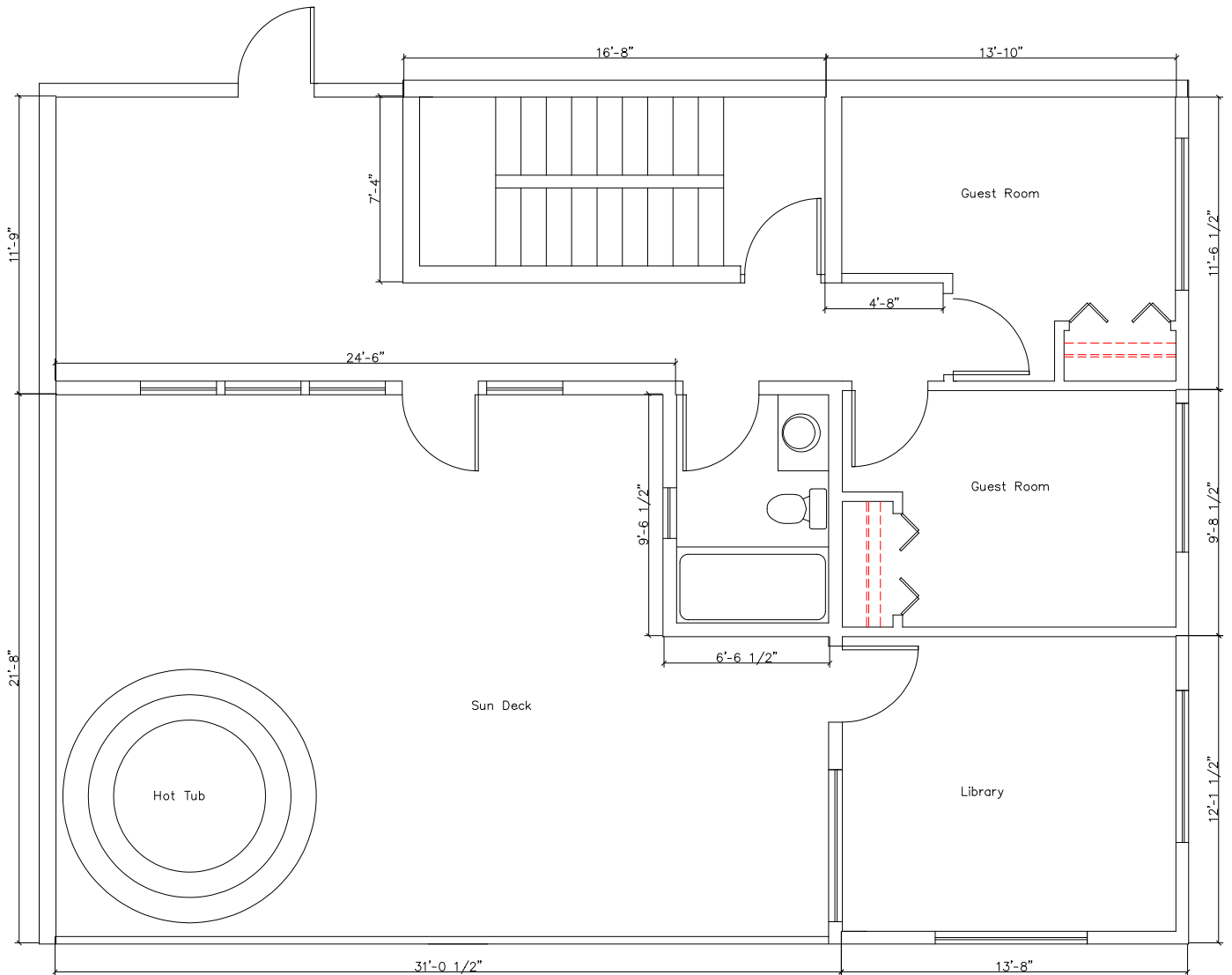
Club House - Upper Level Scale: 1/4"=1'-0"
