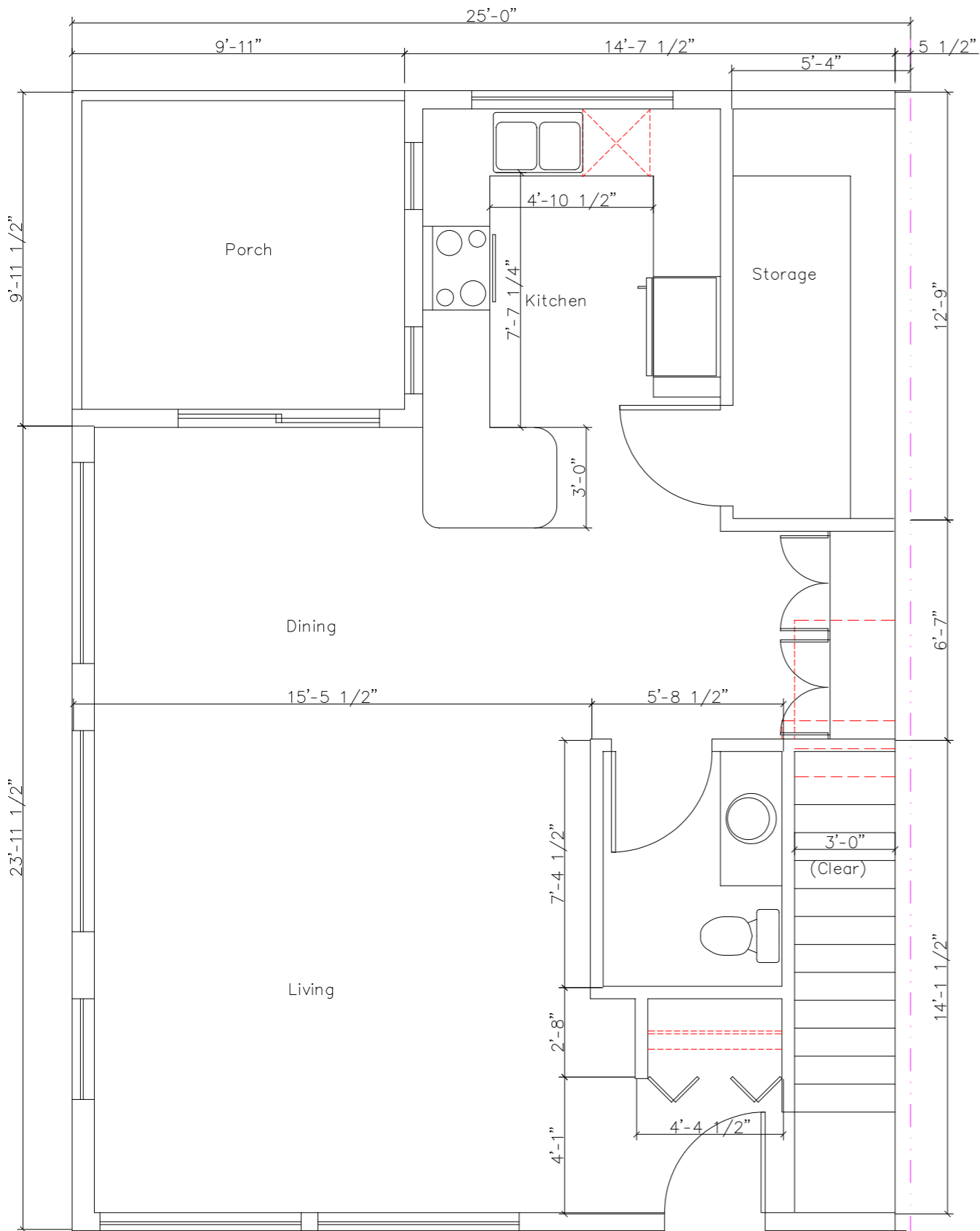
Main Level - Four Bedroom Town House
